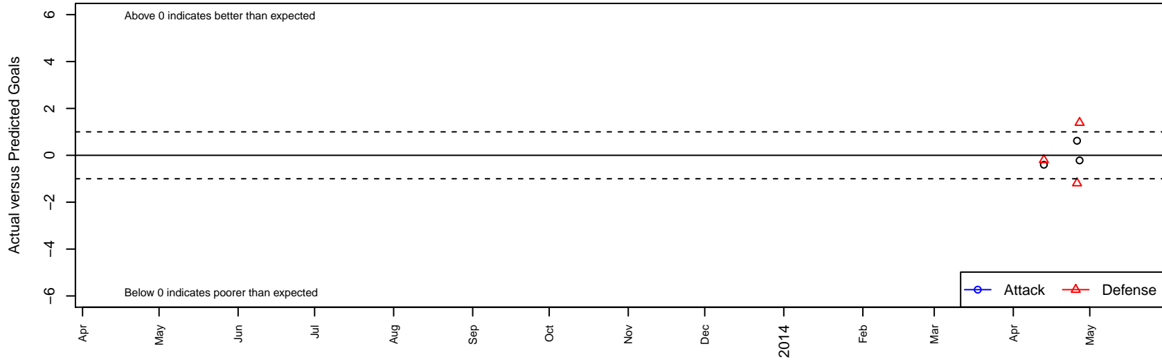
Valley United Fluminense B98 Dots are actual minus expected GF (blue circles) and GA (red triangles). Blue line is smoothed change in attack strength. Red is smoothed change in defense strength.
